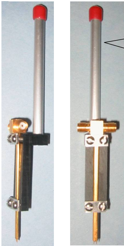
Fully assembled GigaProbes™ GPMMA with Extender Adapter
